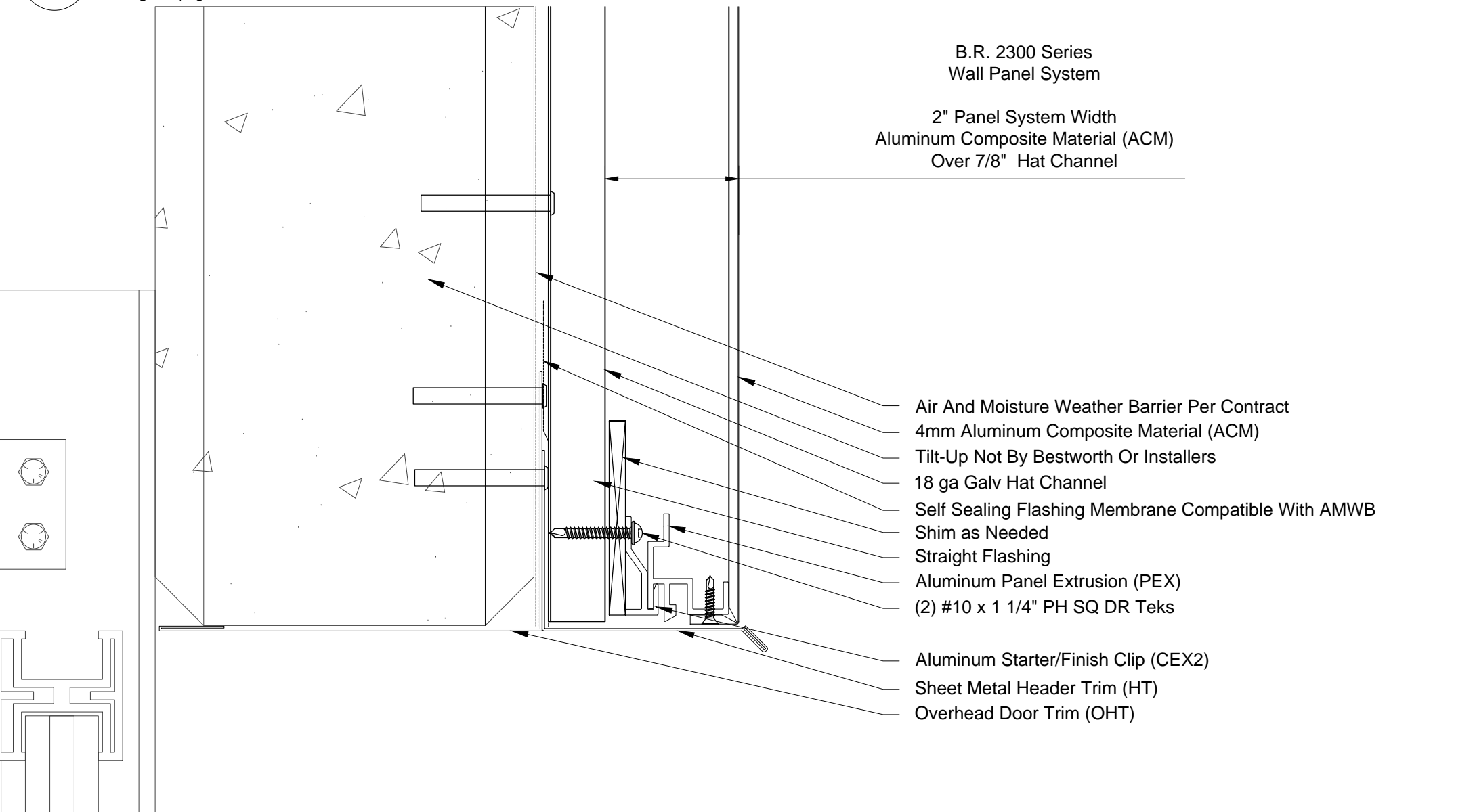
11 2300 ACM @ Overhead Door Header - Tilt Up 6" = 1'-0"
