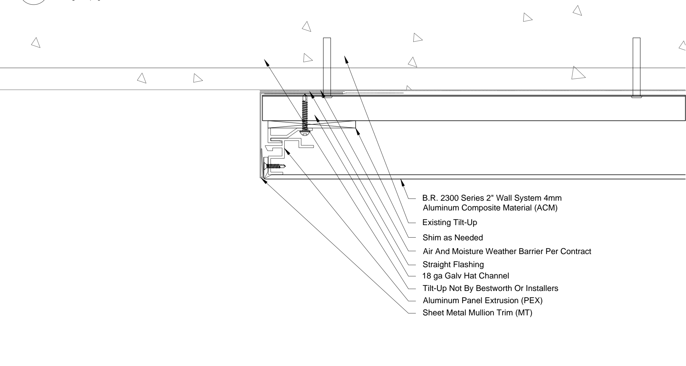
17 2300 ACM @ Termination - Tilt Up 6" = 1'-0"
