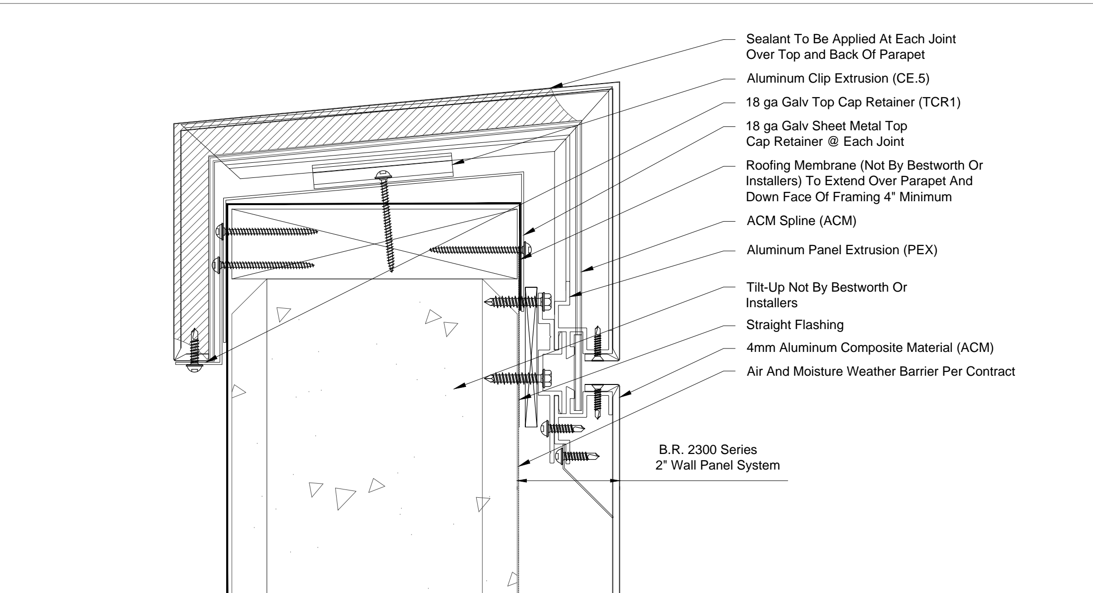
16 2300 ACM @ ACM Top Cap - Tilt Up 6" = 1'-0"
