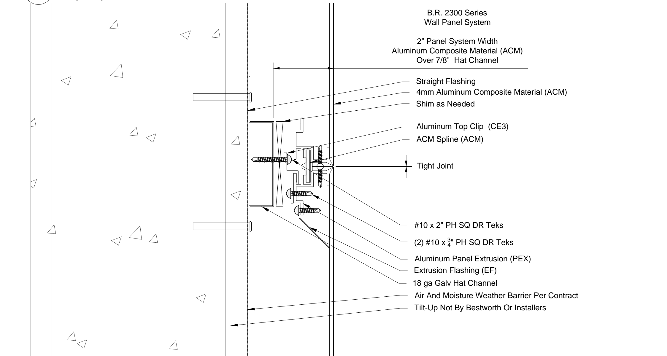
14 2300 ACM @ Tight Panel Joint - Tilt Up 6" = 1'-0"
